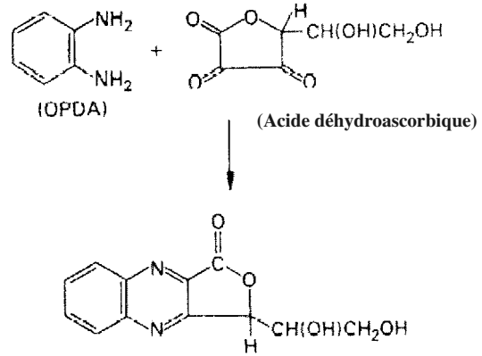
(Oxo-1,2,4-H- dihydroxyethyl-1,2)-3 furo [3,4-b] quinoxaline)
